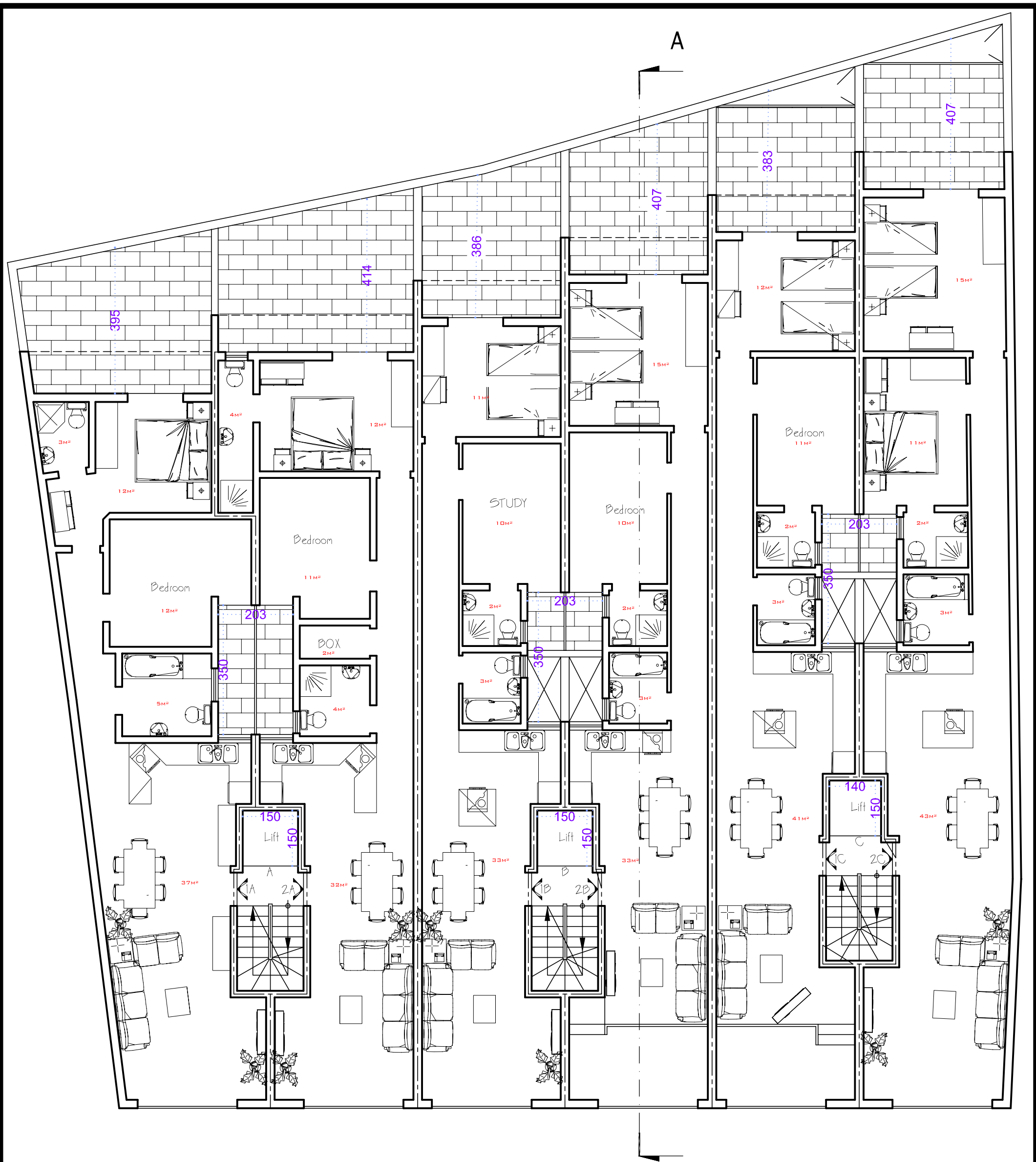
Level 3 Scale 1:100
