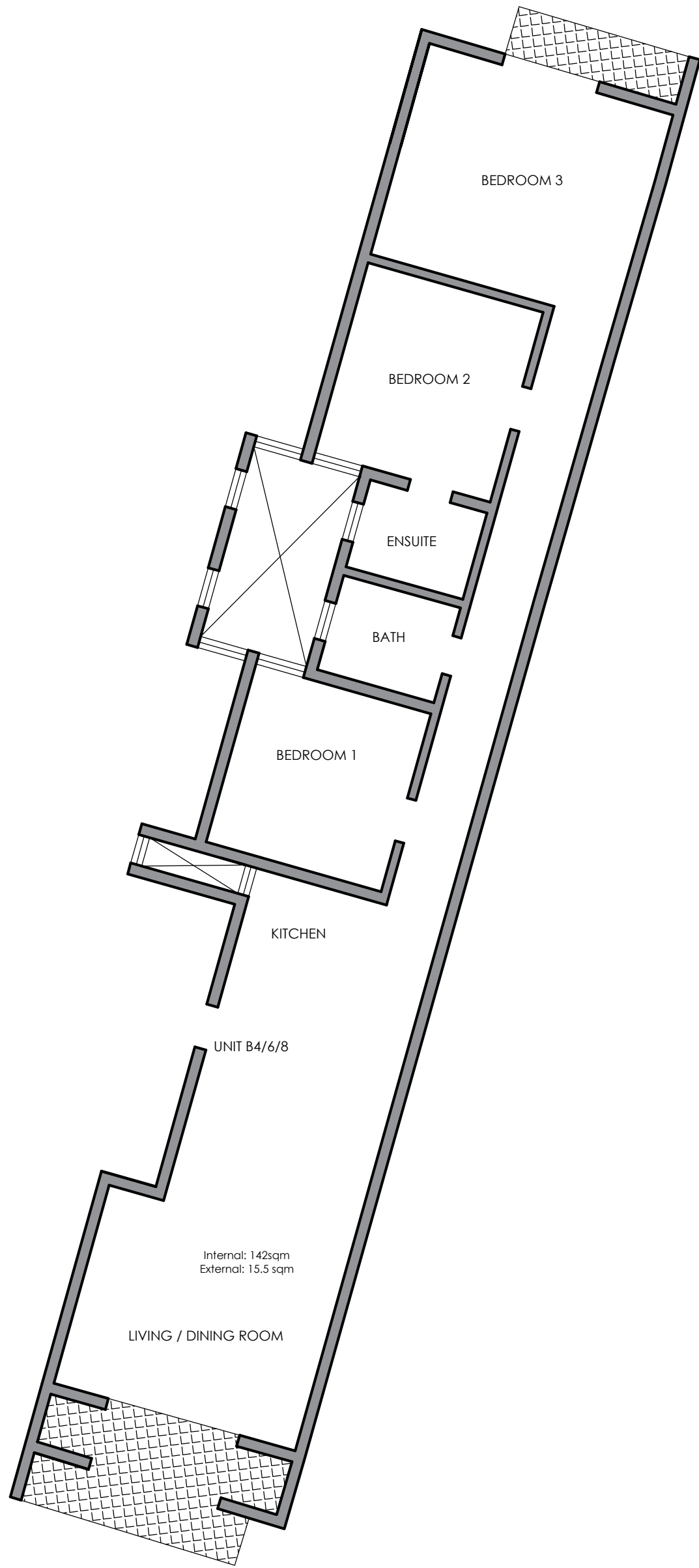
TYPICAL FLOOR (1ST, 2ND & 3RD) - UNIT B4/6/8 PROPOSED SCALE 1:100
