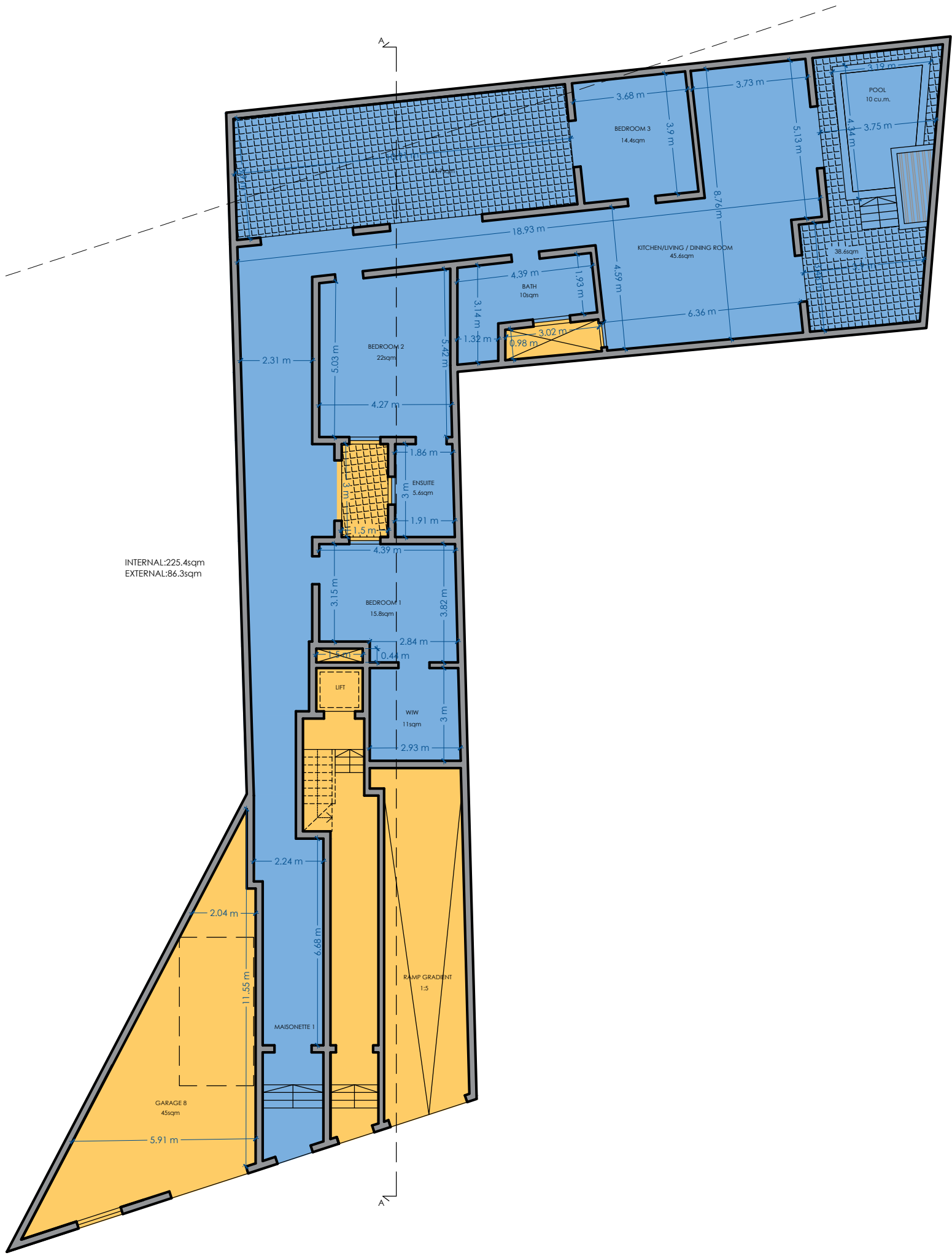
GROUND FLOOR PROPOSED Scale 1:100
